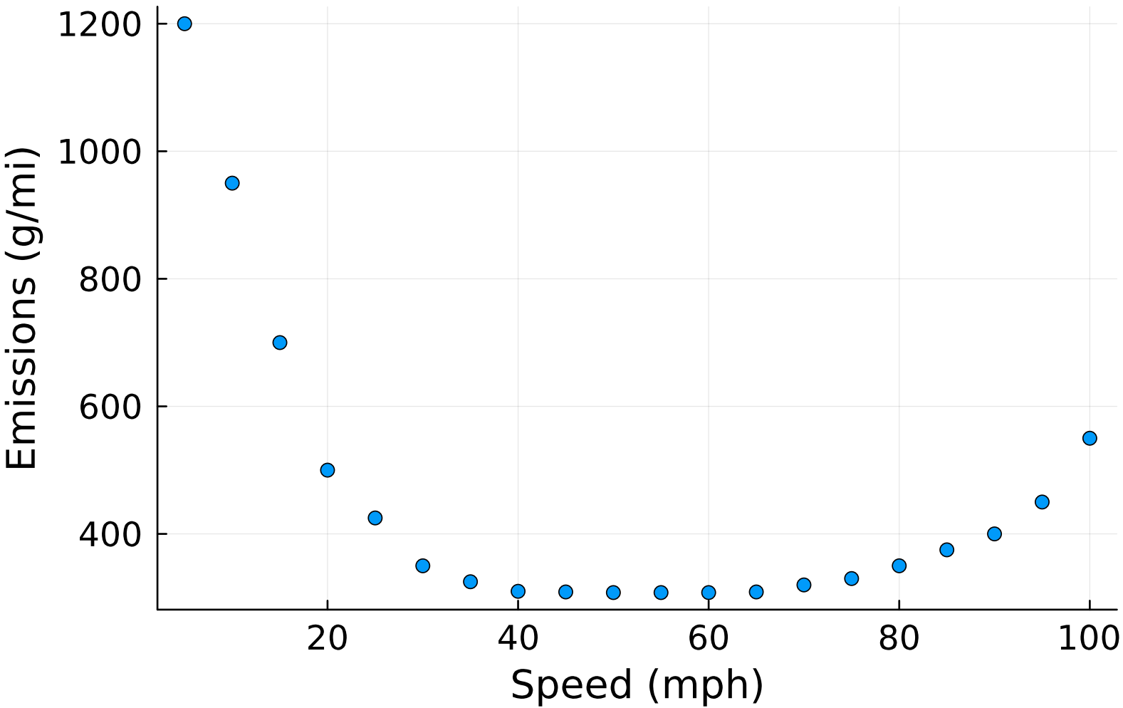
Emissions vs speed — original data
