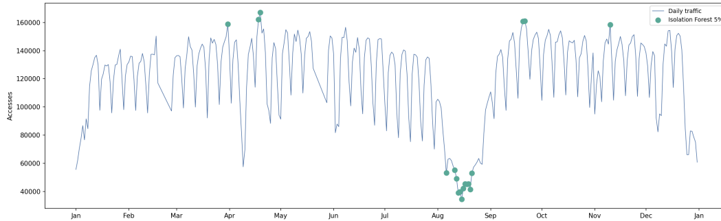
Figure 10: Isolation Forest anomaly detection results.
