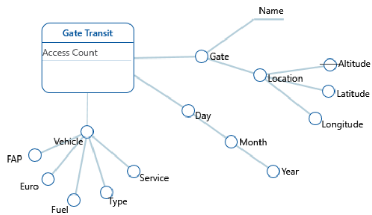
Figure 2: Gate Access DFM
