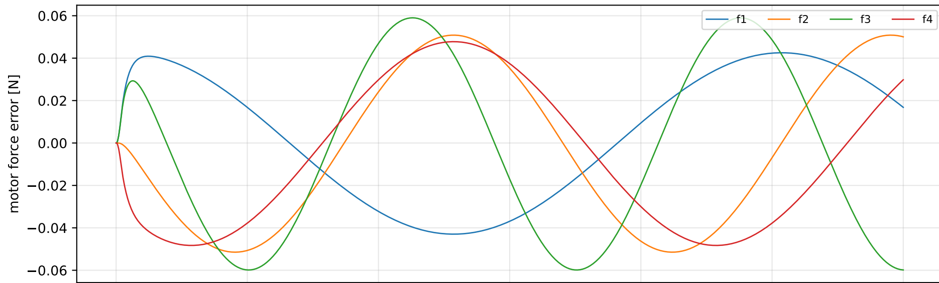
RotorMotor plugin minus direct force actuator
