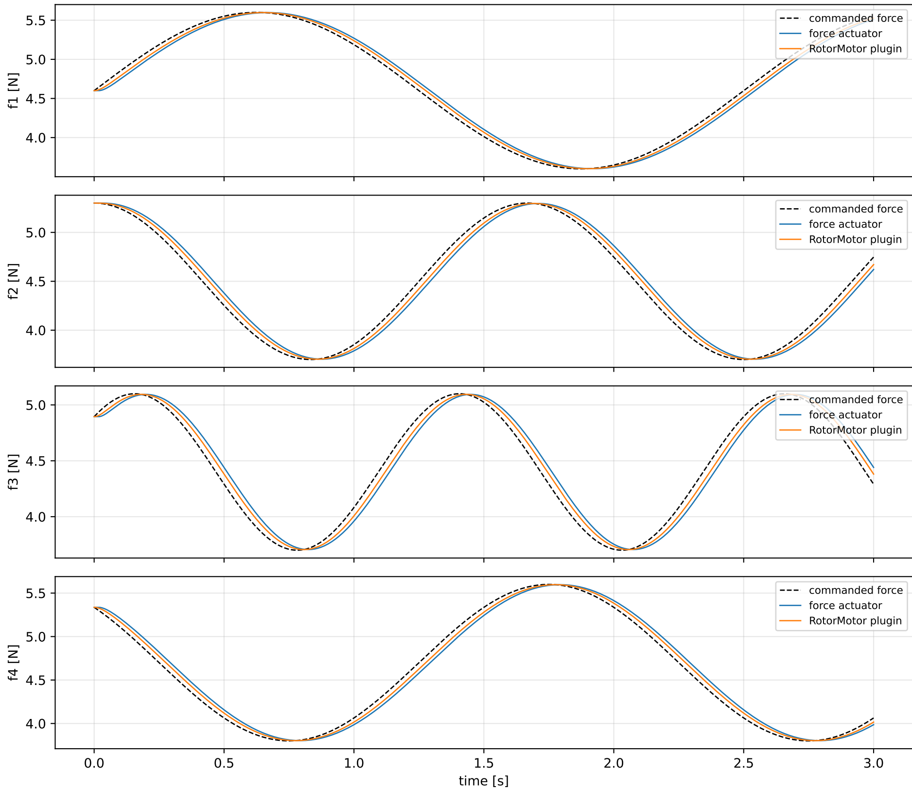
Per-motor thrust comparison
