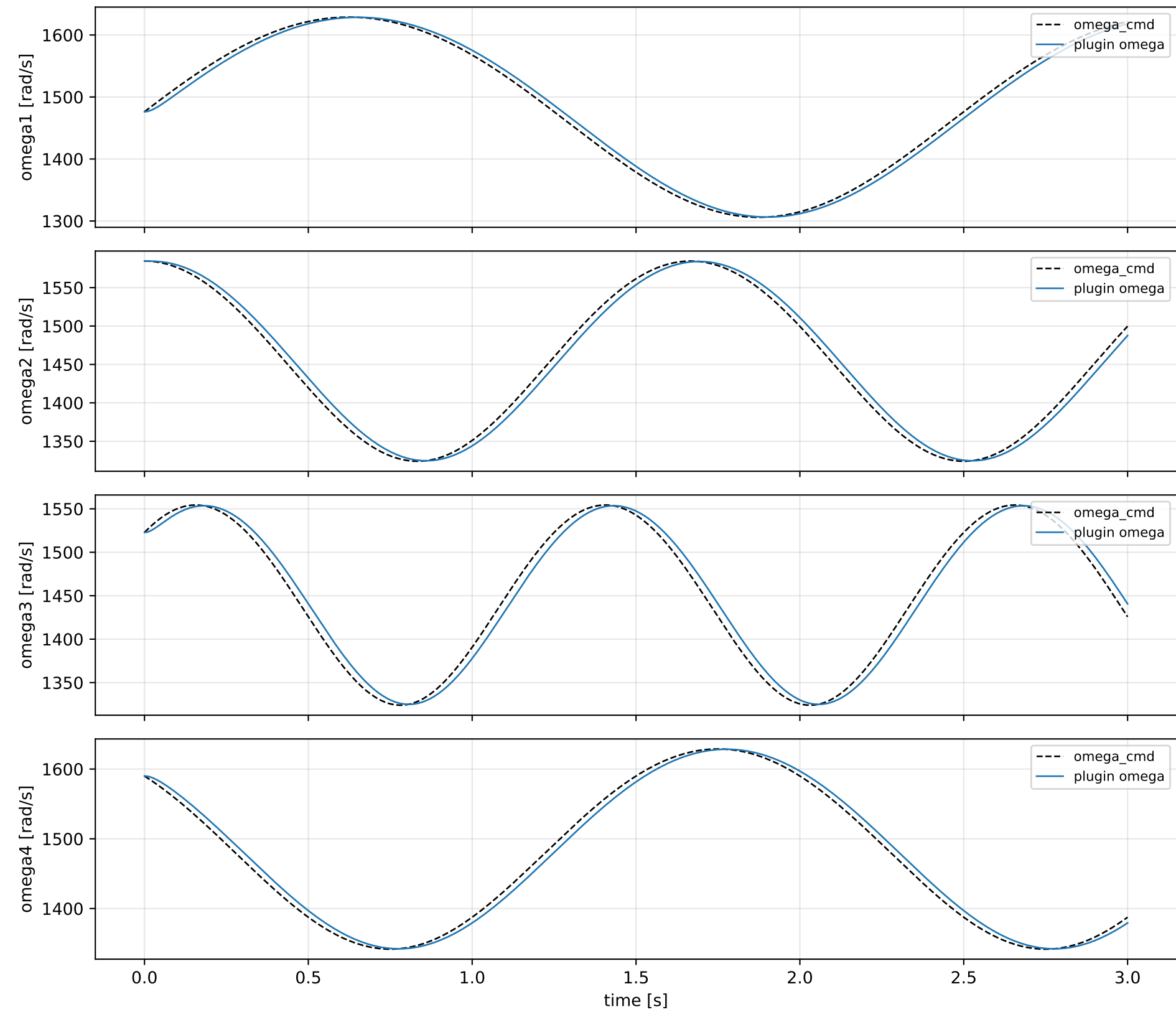
RotorMotor speed state
