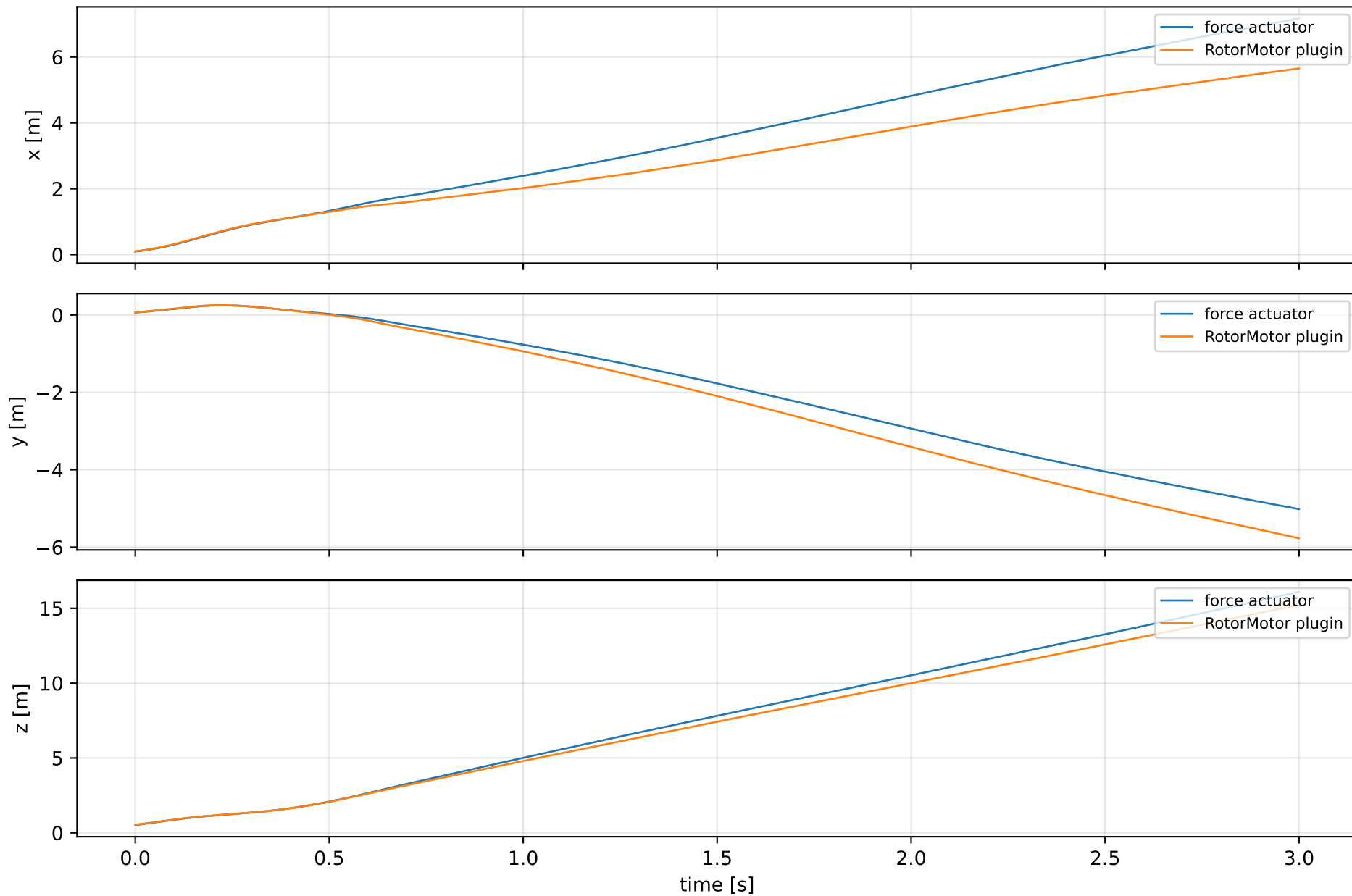
Free-body position under actuator outputs
