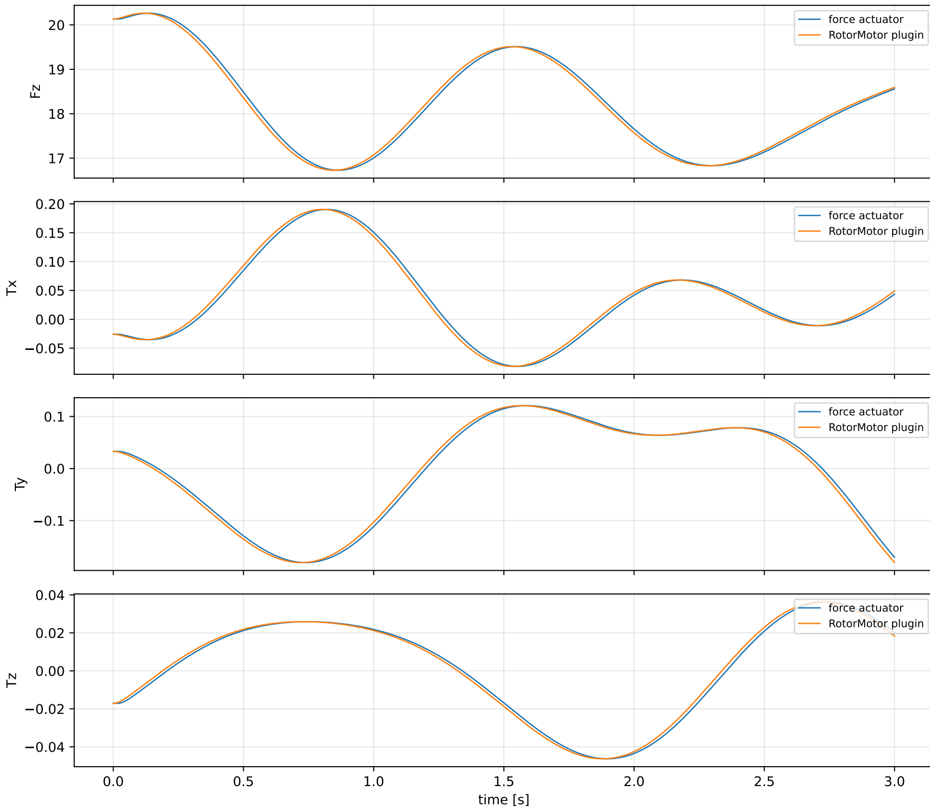
Aggregate body wrench from actuator_force
