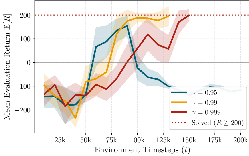
Figure 4: Evaluation reward progression for different discount factors \gamma .
