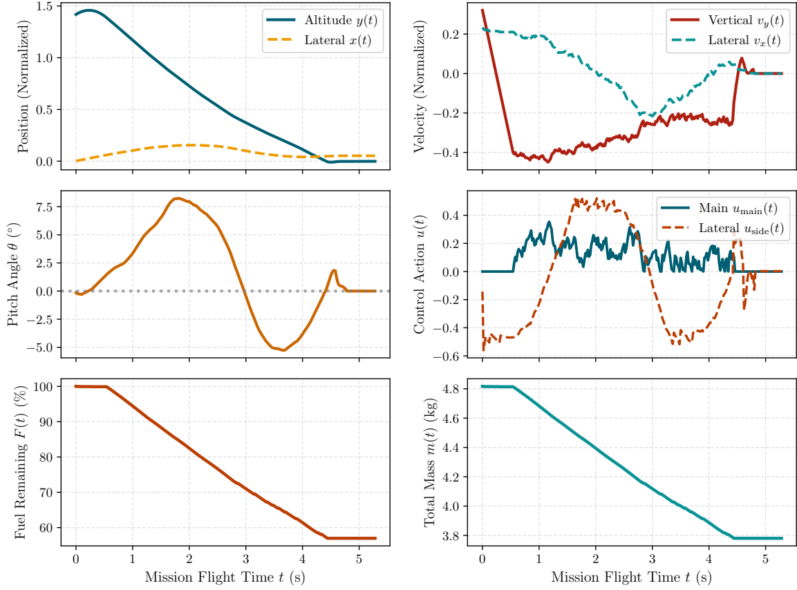
Figure 7: Time history of a representative closed-loop landing flight: position, velocity, pitch angle, mass depletion, and continuous throttle commands.
