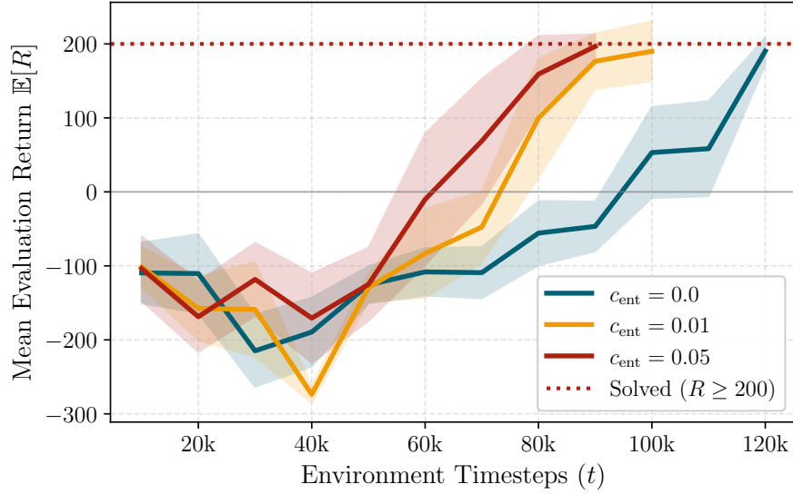
Figure 5: Evaluation reward progression for different entropy regularization coefficients c_{\text{ent}} .
