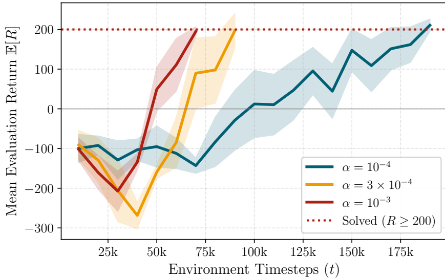
Figure 3: Evaluation reward progression for different learning rates \alpha , with their respective \pm 1\sigma confidence bands.
