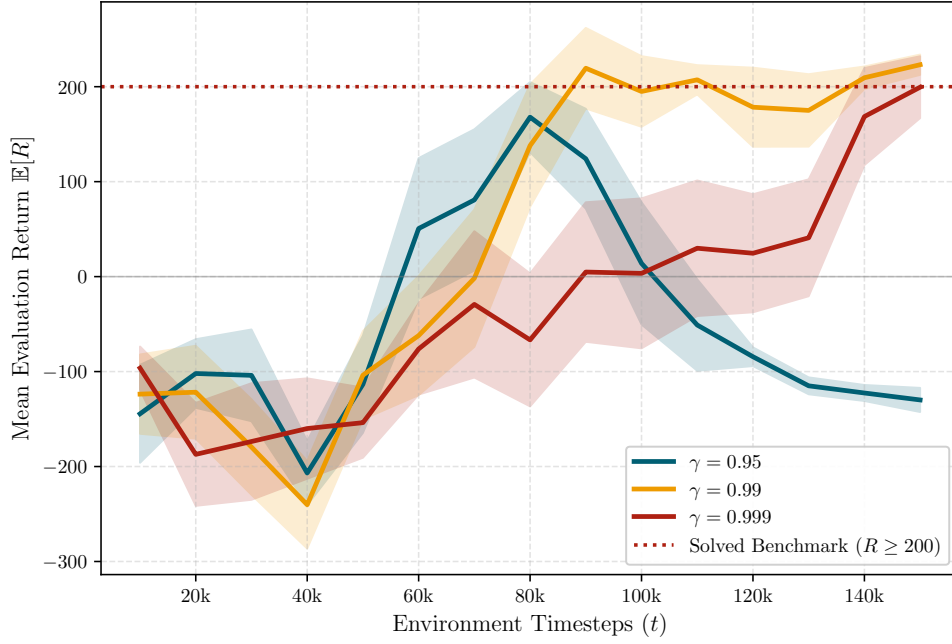
Figure 4: Evaluation reward progression for different discount factors \gamma .
