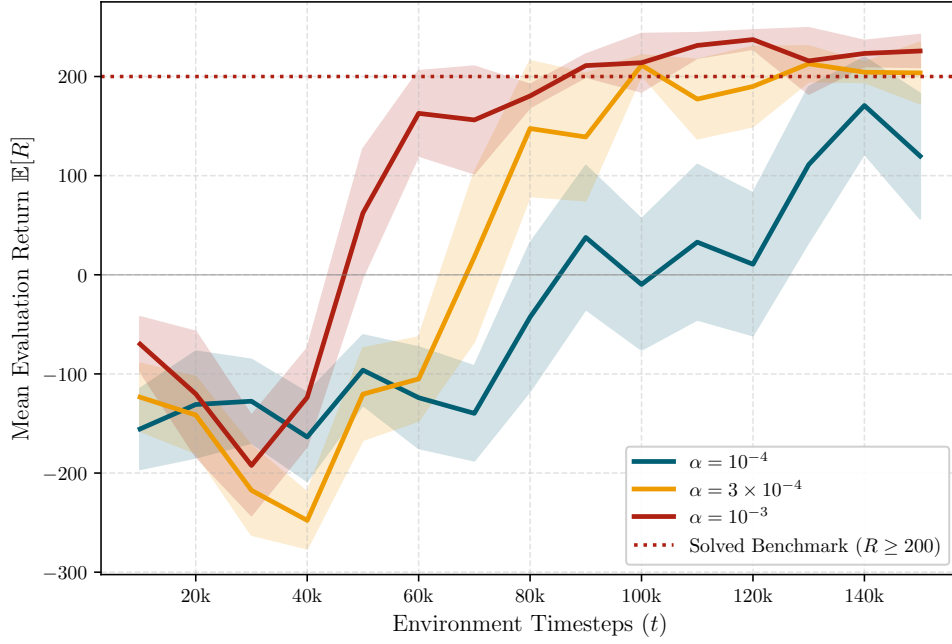
Figure 3: Evaluation reward progression for different learning rates \alpha , with their respective \pm 1\sigma confidence bands.
