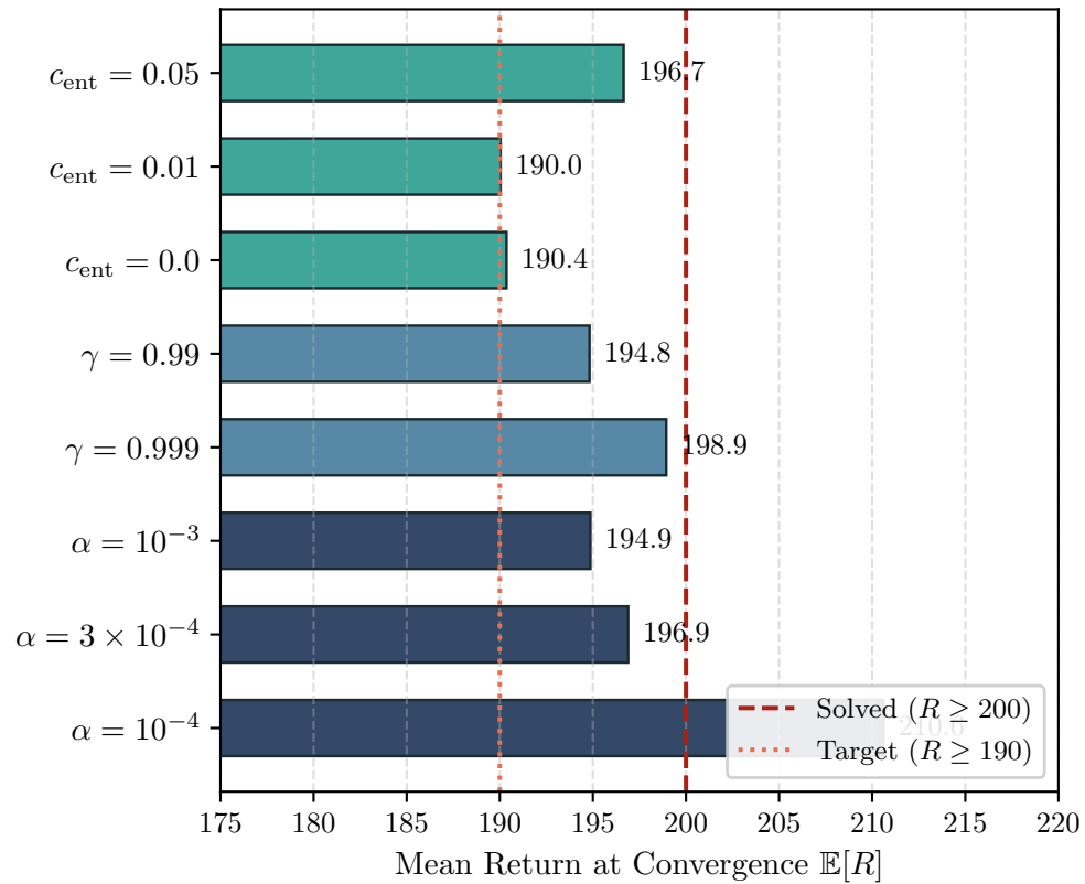
Convergence Quality: Final Return
