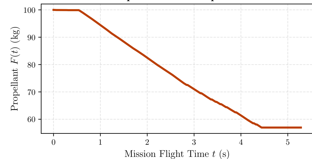
Propellant Mass Depletion
