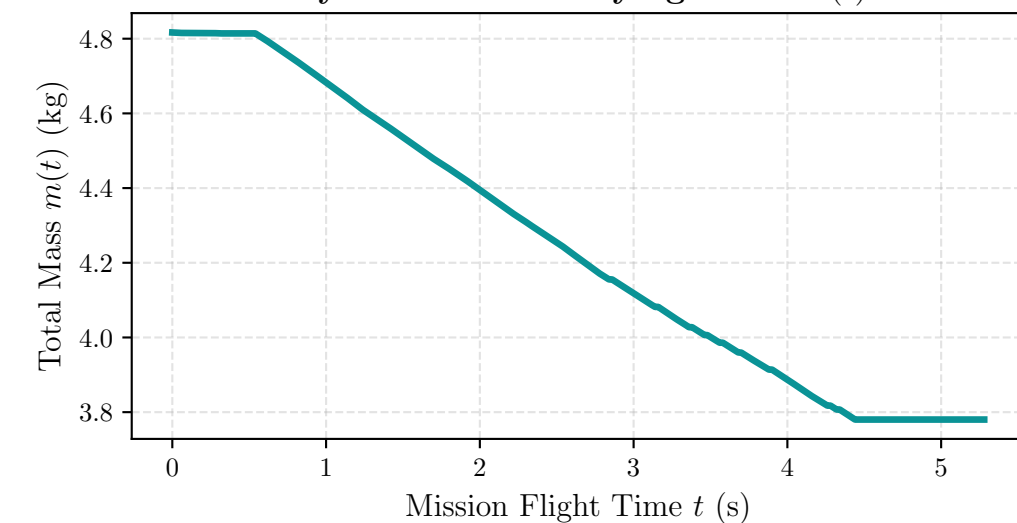
Dynamic Mass-Varying State m(t)
