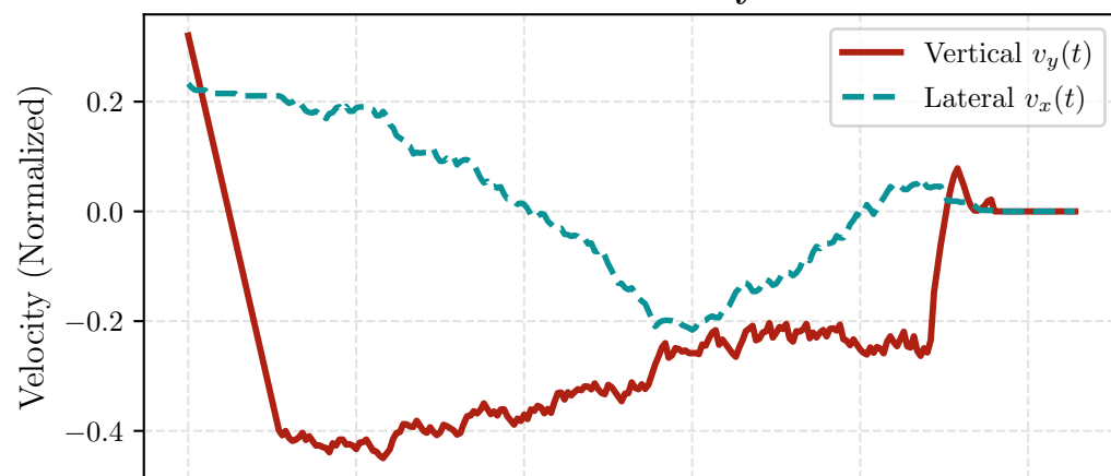
Translational Velocity Profiles
