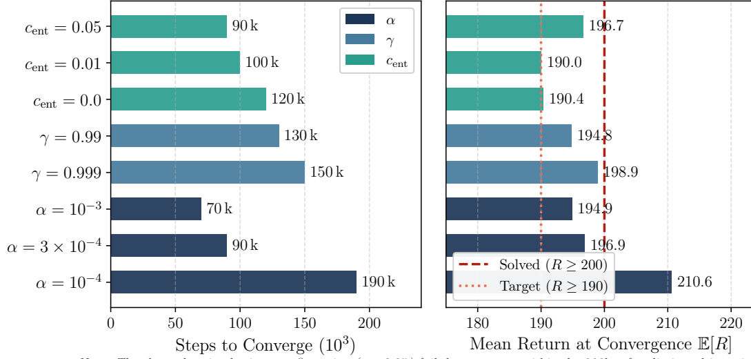
Figure 6: Comparison of training steps and mean return to achieve certified convergence across hyperparameter configurations.
