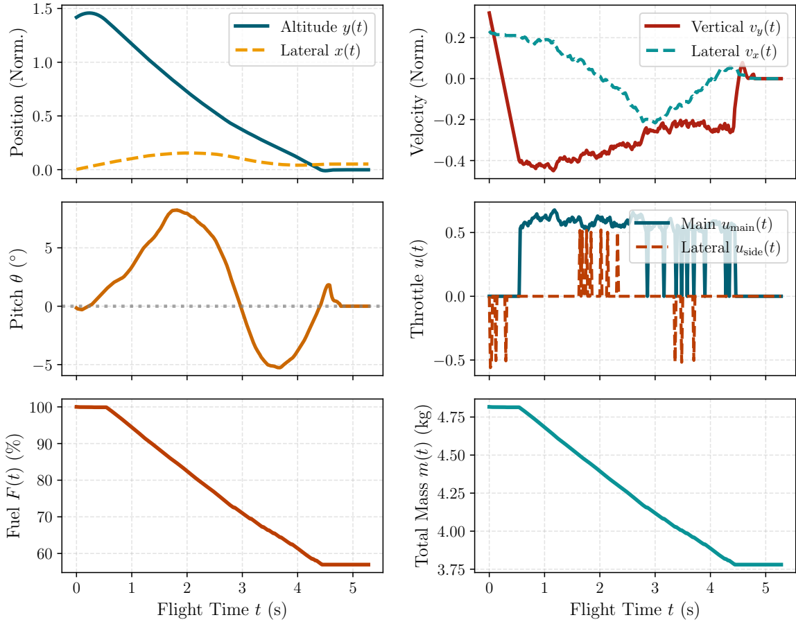
Figure 7: Time history of a representative closed-loop landing flight: position, velocity, pitch angle, mass depletion, and continuous throttle commands.
