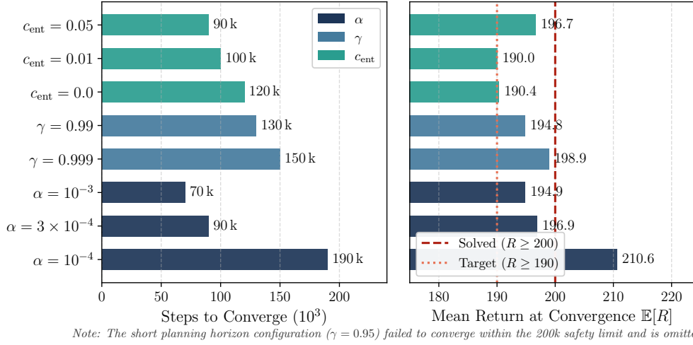
Figure 6: Comparison of training steps and mean return to achieve certified convergence across hyperparameter configurations.
