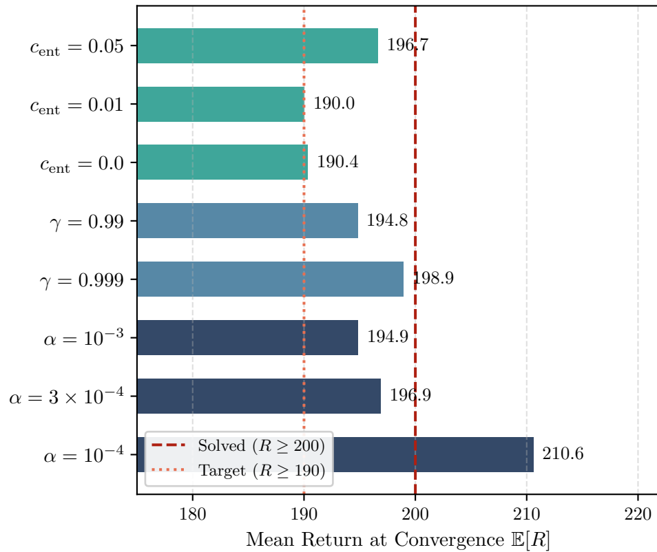
Convergence Quality: Final Return
