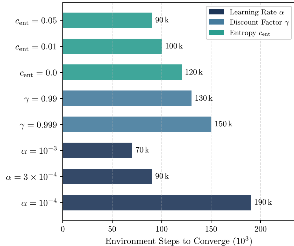
Sample Efficiency: Steps to Convergence
