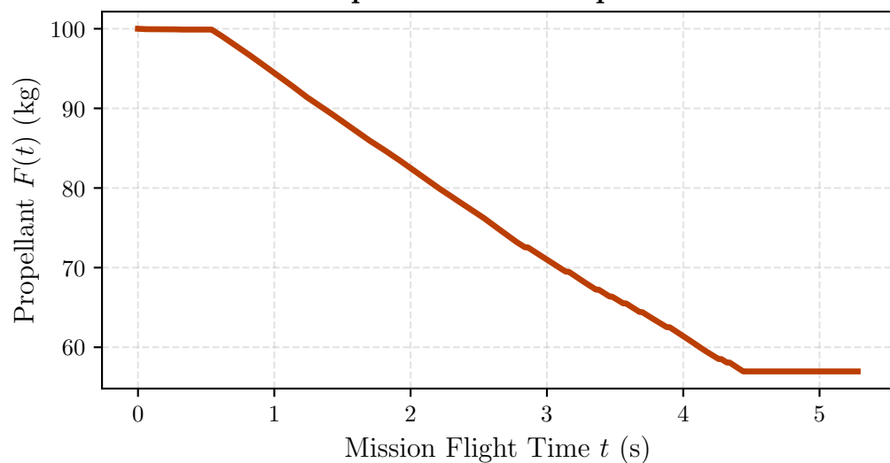
Propellant Mass Depletion
