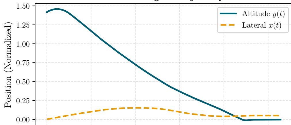
Lander Flight Trajectory
