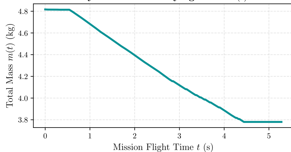
Dynamic Mass-Varying State m(t)
