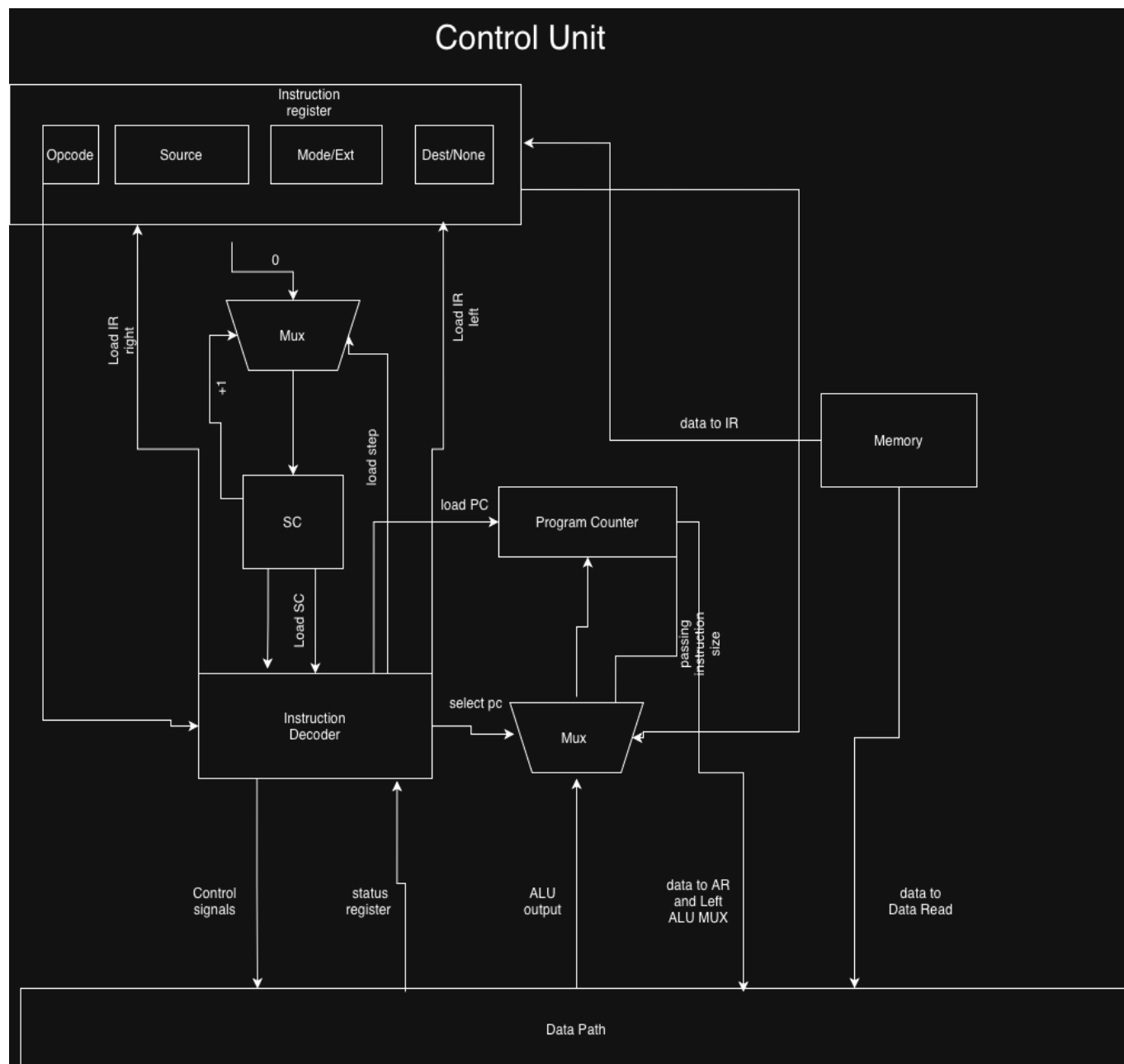
Рис. 1: Control Unit
