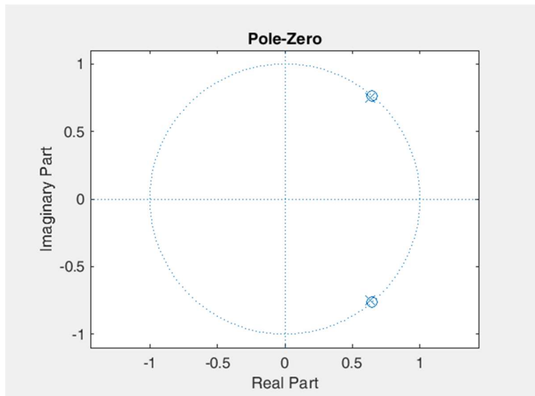
Fig 2.8: Pole-zero diagram for Chebyshev Type II
