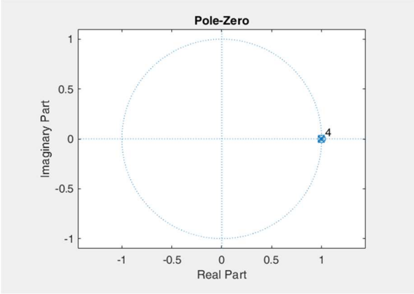
Fig 2.4: Pole-zero diagram for Butterworth
