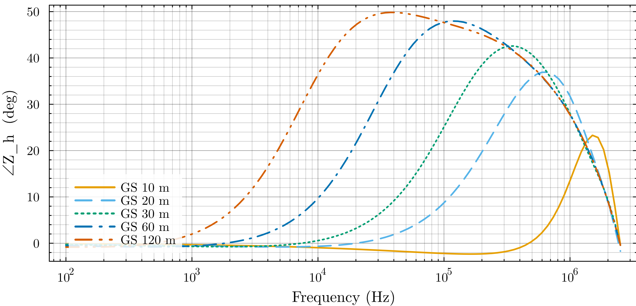
Harmonic Impedance — Phase
