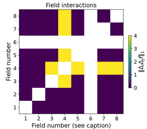
bitnami/apache 7 measured changes; 21 pairs (complete)
