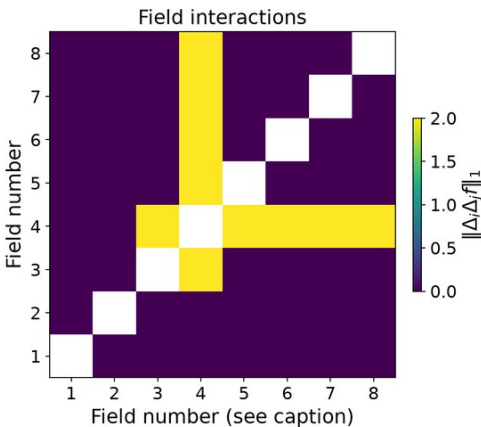
bitnami/whereabouts 8 measured changes; 28 pairs (complete)
