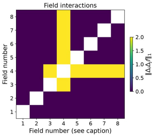
bitnami/cadvisor 8 measured changes; 28 pairs (complete)
