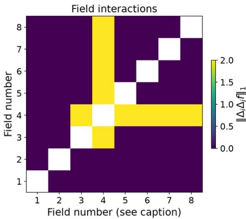
bitnami/multus-cni 8 measured changes; 28 pairs (complete)
