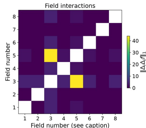
bitnami/fluent-bit 8 measured changes; 28 pairs (complete)
