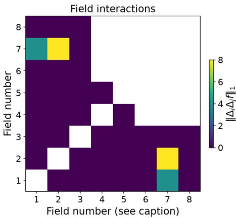
bitnami/flux 8 measured changes; 19 pairs (time-limit)
