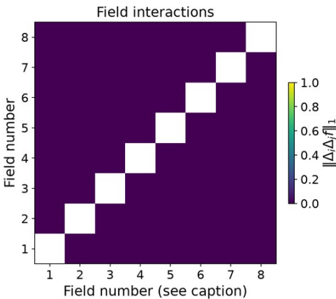
bitnami/victoriametrics 8 measured changes; 28 pairs (complete)
