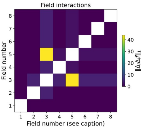
bitnami/consul 8 measured changes; 28 pairs (complete)
