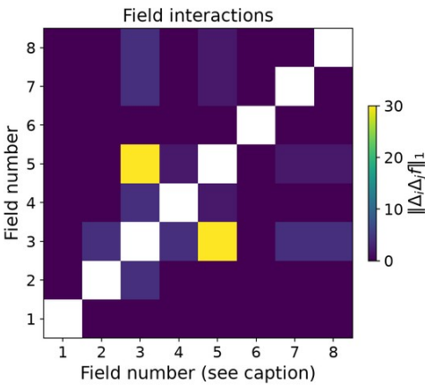
bitnami/memcached 8 measured changes; 28 pairs (complete)
