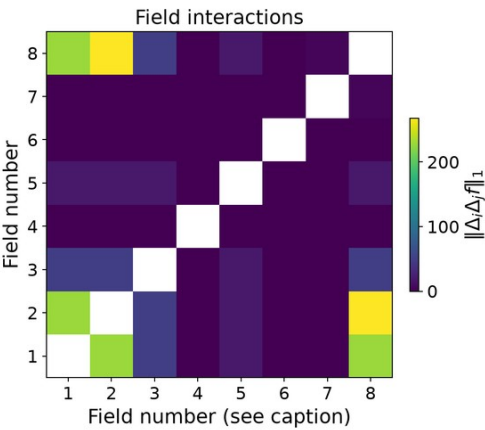
bitnami/kube-state-metrics 8 measured changes; 28 pairs (complete)
