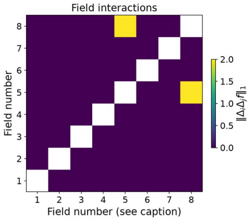
bitnami/vault 8 measured changes; 28 pairs (complete)
