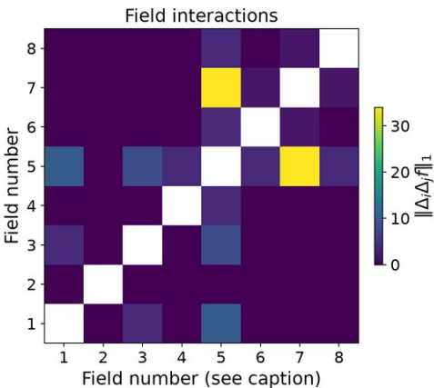
bitnami/logstash 8 measured changes; 28 pairs (complete)
