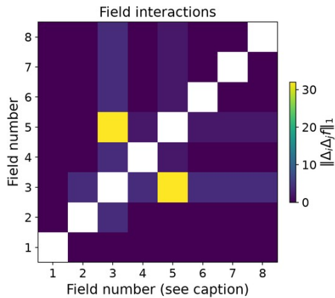
bitnami/haproxy 8 measured changes; 28 pairs (complete)
