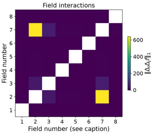
bitnami/redis-cluster 8 measured changes; 28 pairs (complete)
