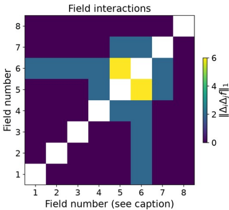
bitnami/flink 8 measured changes; 28 pairs (complete)
