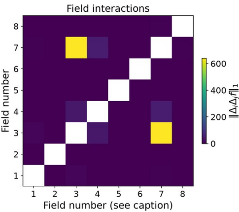
bitnami/valkey-cluster 8 measured changes; 28 pairs (complete)
