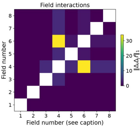
bitnami/kubernetes-event-exporter 8 measured changes; 28 pairs (complete)
