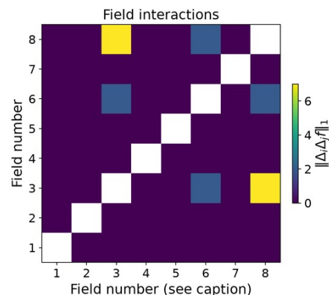
bitnami/fluentd 8 measured changes; 28 pairs (complete)
