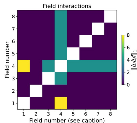
bitnami/grafana-k6-operator 8 measured changes; 28 pairs (complete)
