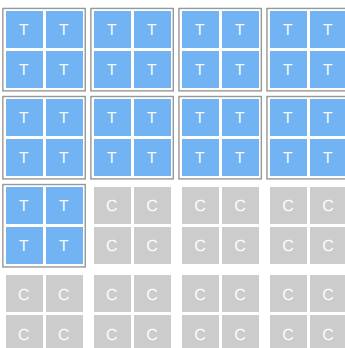
Cluster
