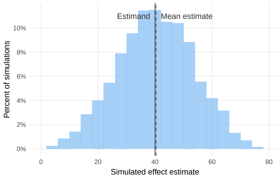
Figure 1: Figure 9.1: Sampling distribution of estimates
