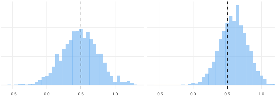
Matched difference-in-means
