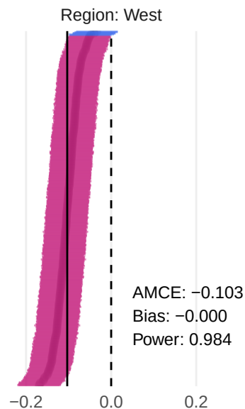
AMCE estimate and 95% confidence interval
