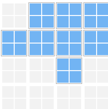
Cluster
