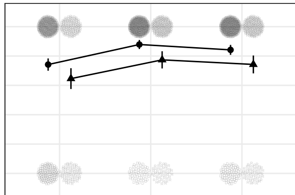
Lucid Replication
