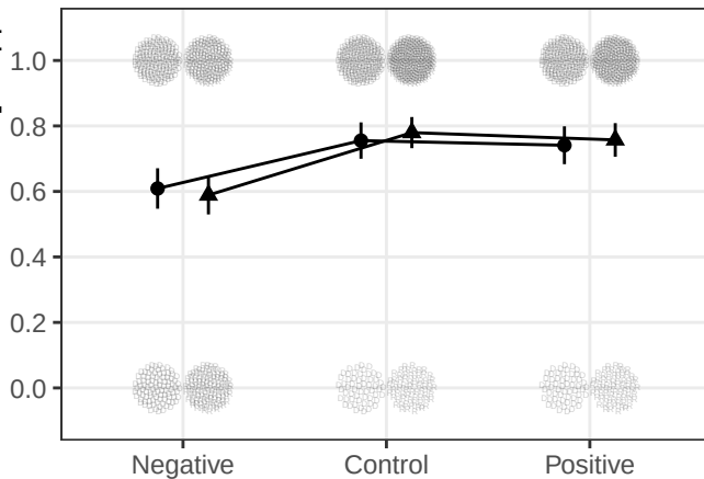
GfK Replication
