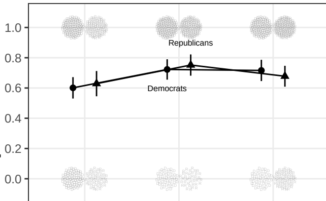
GfK Replication
