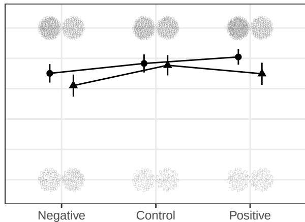
Lucid Replication
