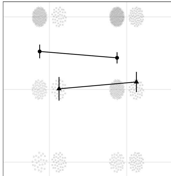
Mechanical Turk Replication
