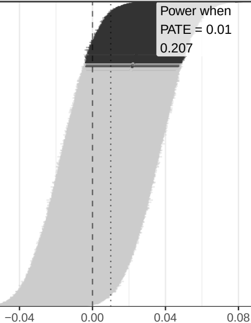
Simulated OLS estimate
