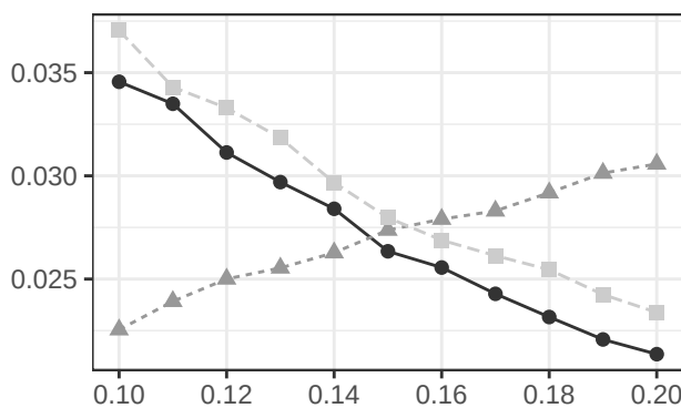
RMSE of best arm
