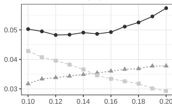
RMSE of ATE
