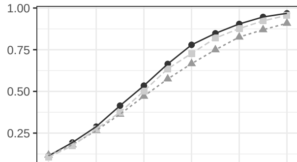
Best arm selection
