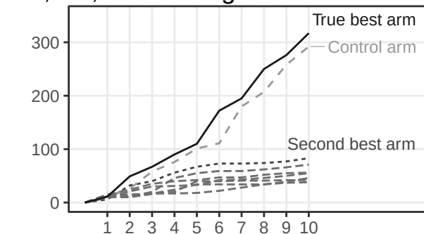
Case 3: Competing second best, TS, control augmented
