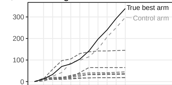
Case 2: No clear winner, TS, control augmented
