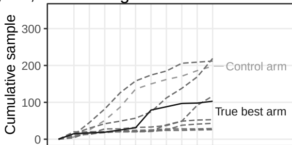
Case 3: Competing second best, TS, control augmented
