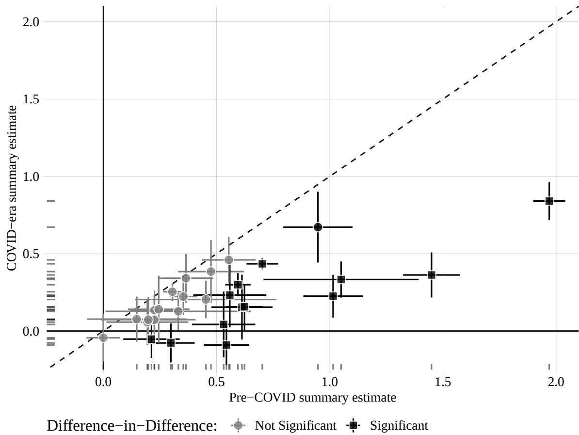
Figure 2: Comparison of 28 summary effect sizes across 11 studies, conjoint excluded. Fill marks a difference significant at p < 0.05 ; square points remain significant after controlling the false discovery rate.
