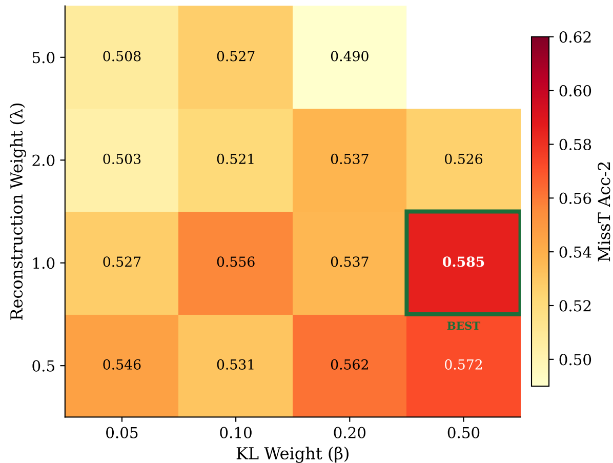
MissT: KL × Recon Interaction
