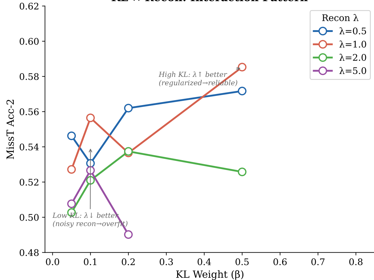
KL × Recon: Interaction Pattern
