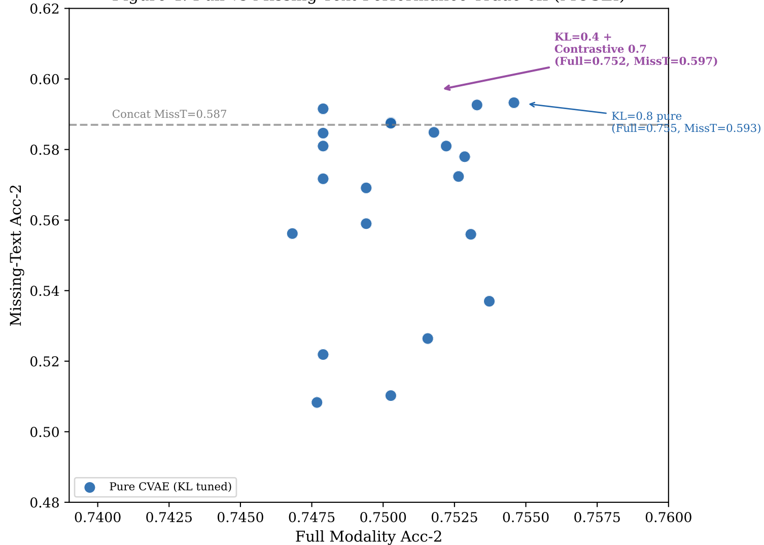
Figure 4: Full vs Missing-Text Performance Trade-off (MOSEI)
