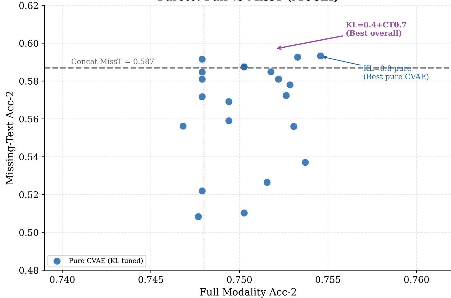
Pareto: Full vs MissT (MOSEI)
