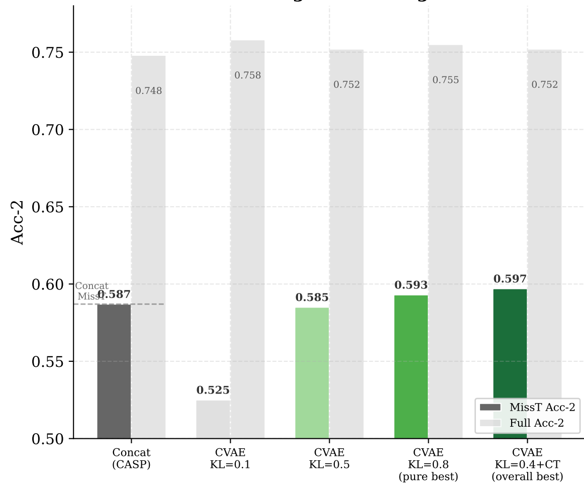
MOSEI: Configuration Progression
