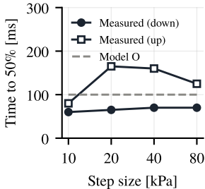
(a) Isolated steps
