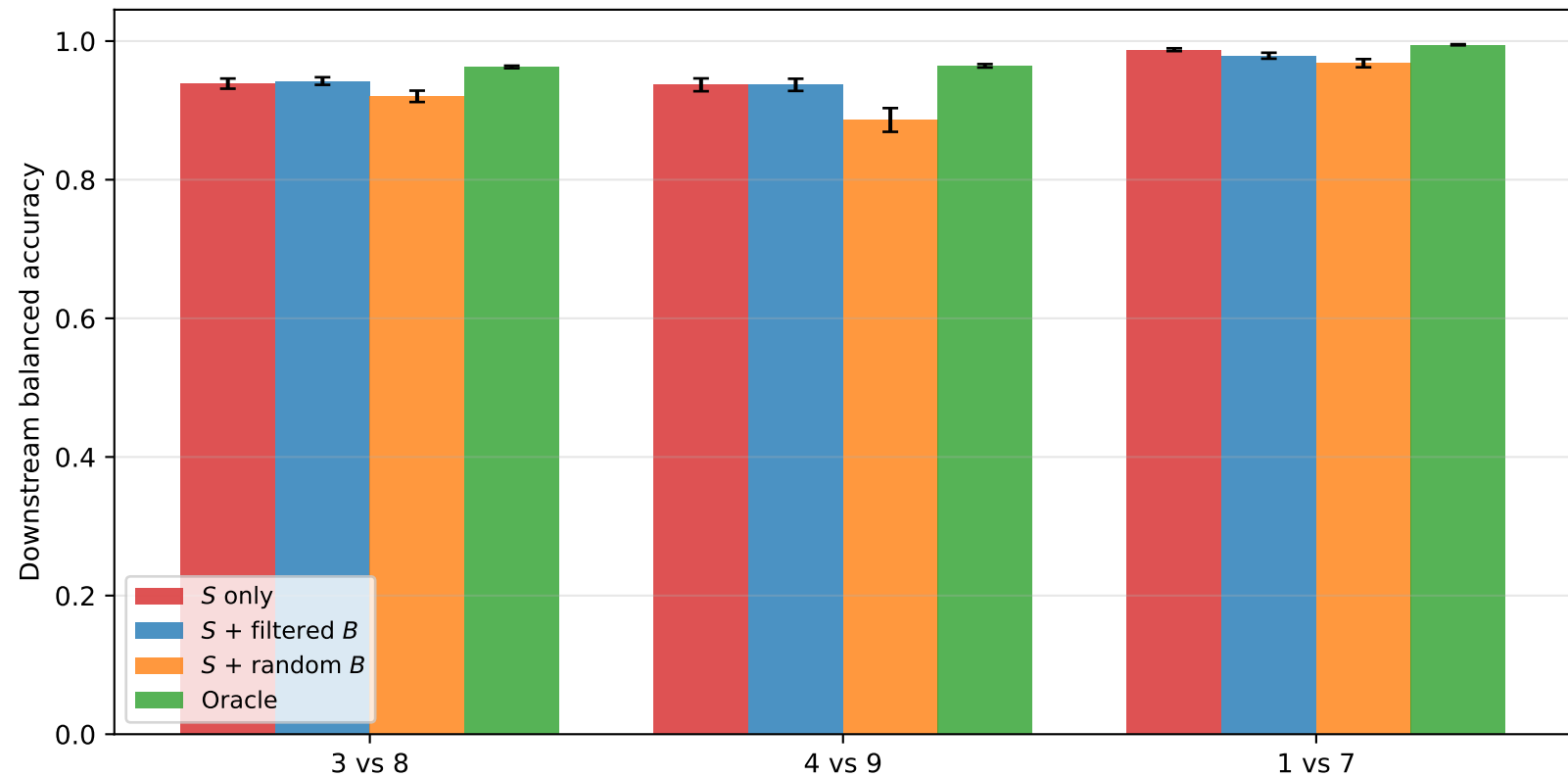
MNIST: filtering improves within-S digit classification ( N_S = 200 )
