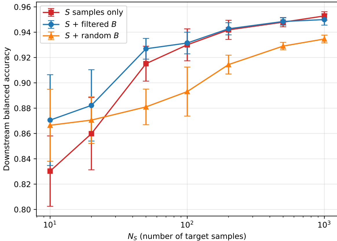
MNIST (3 vs 8): accuracy vs N_S
