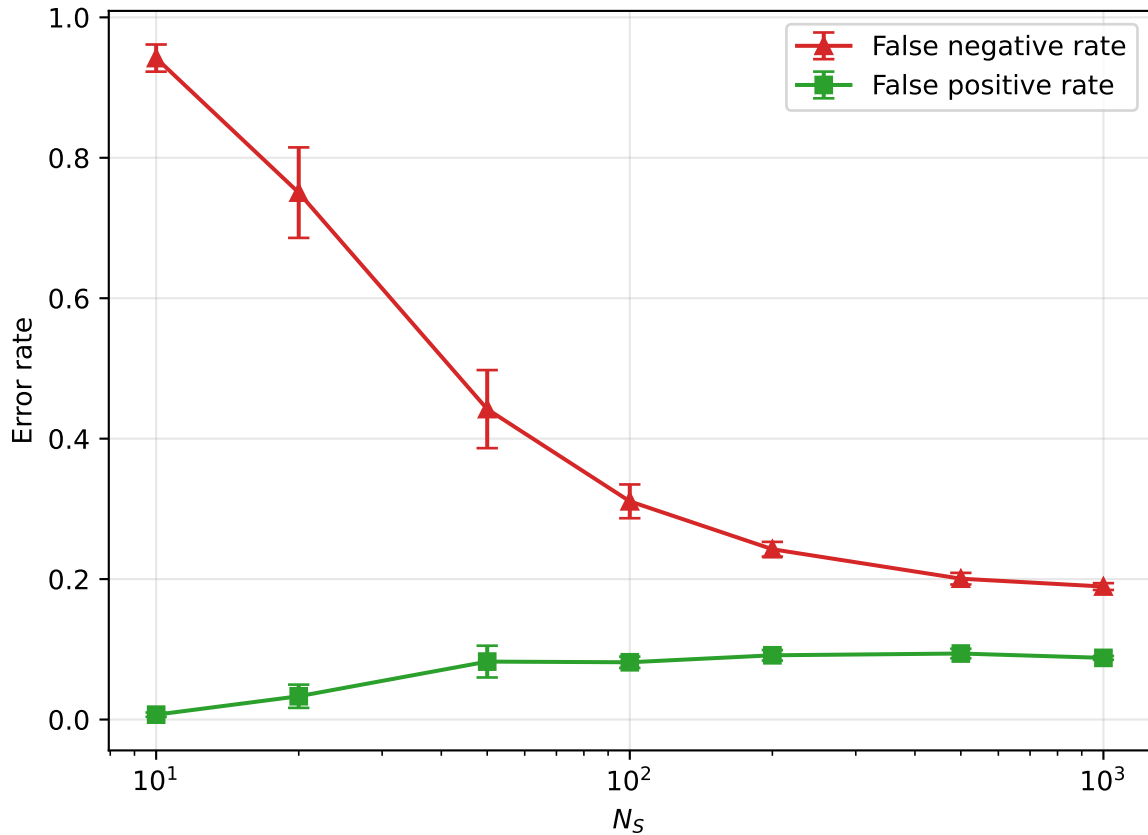
MNIST (3 vs 8): filter errors vs N_S
