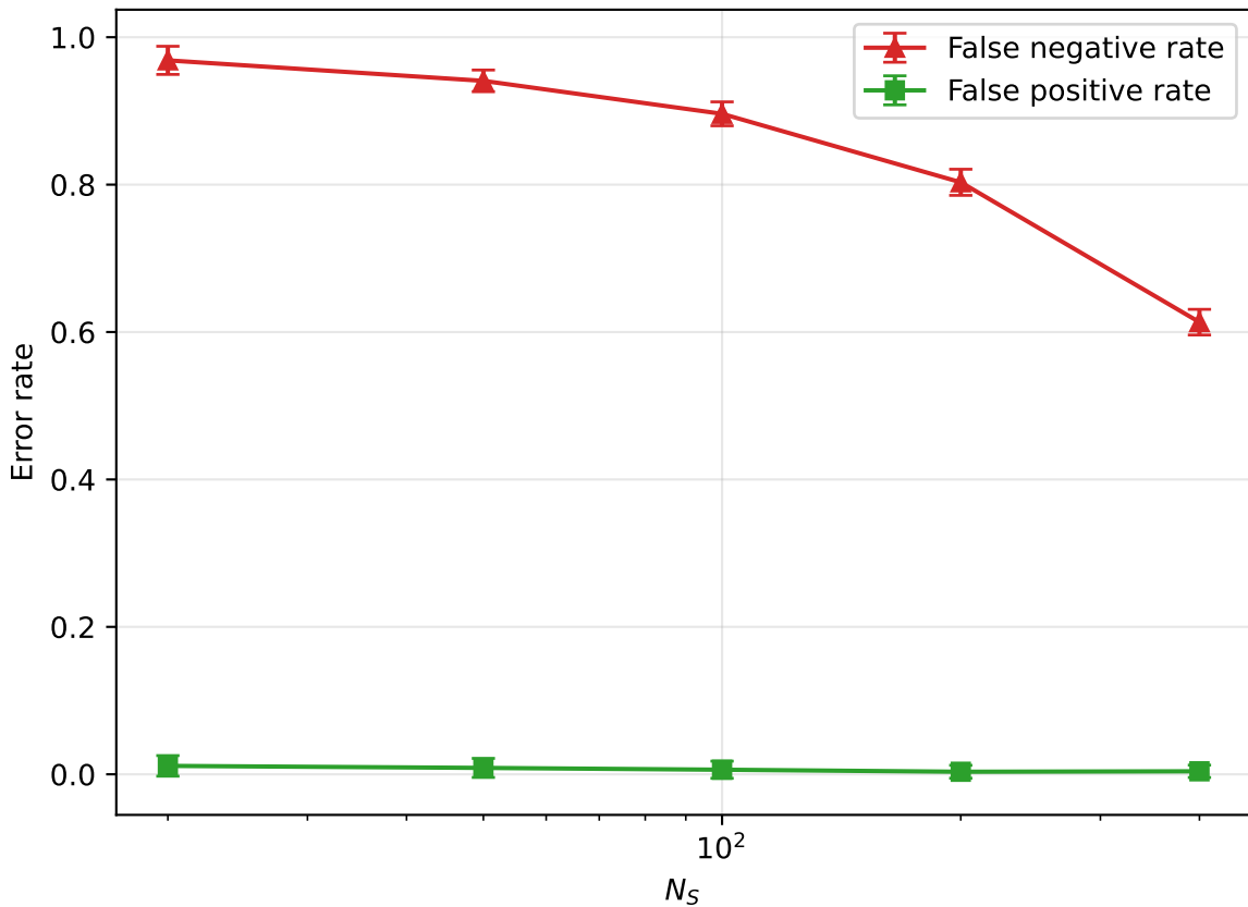
20 Newsgroups (baseball vs hockey): filter errors vs N_S
