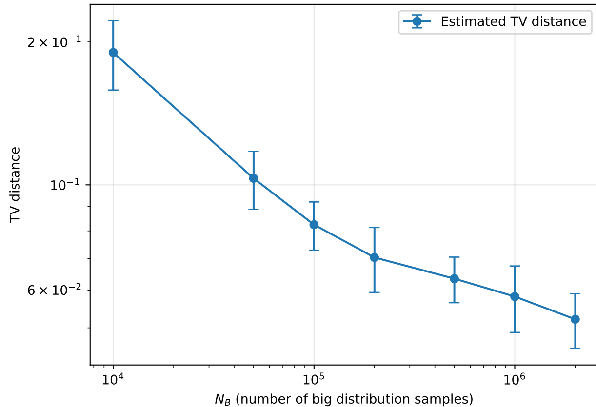
TV distance vs N_B ( N_S = 1000 , p = 0.01 )
