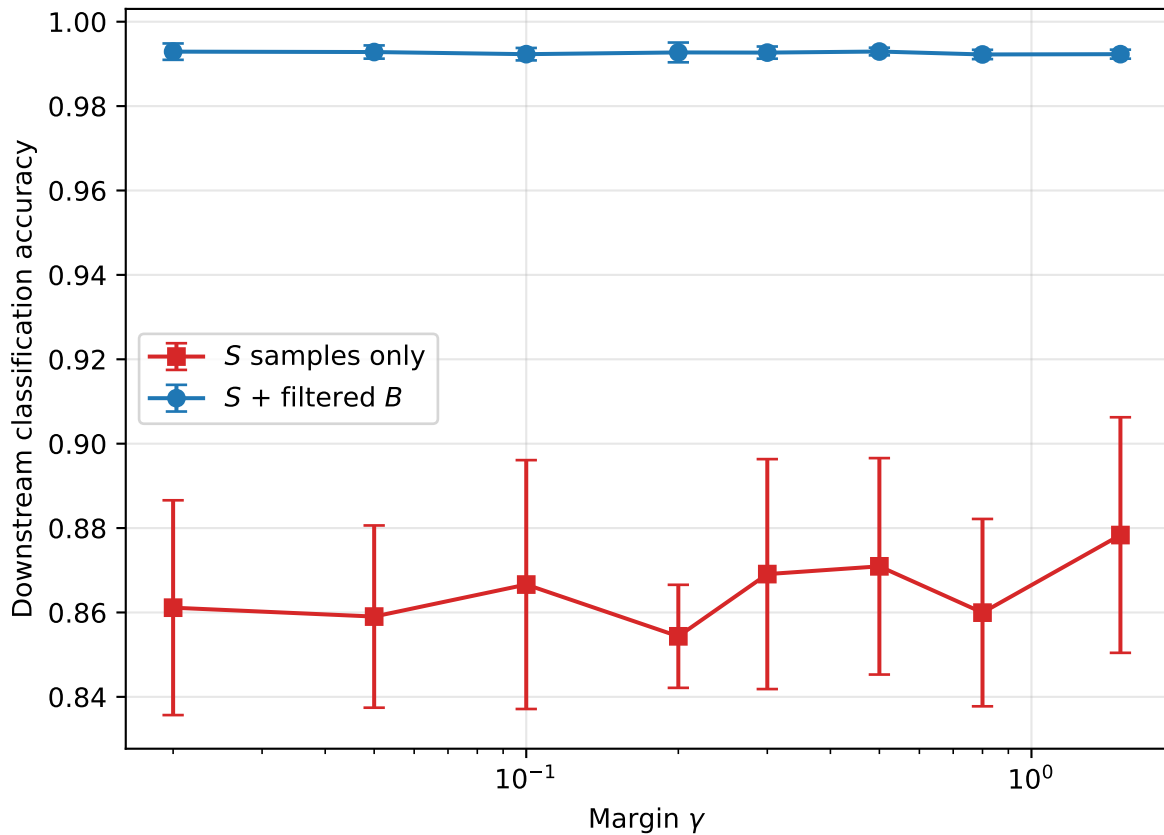
Downstream accuracy vs \gamma ( N_S = 30, p = 0.01 )
