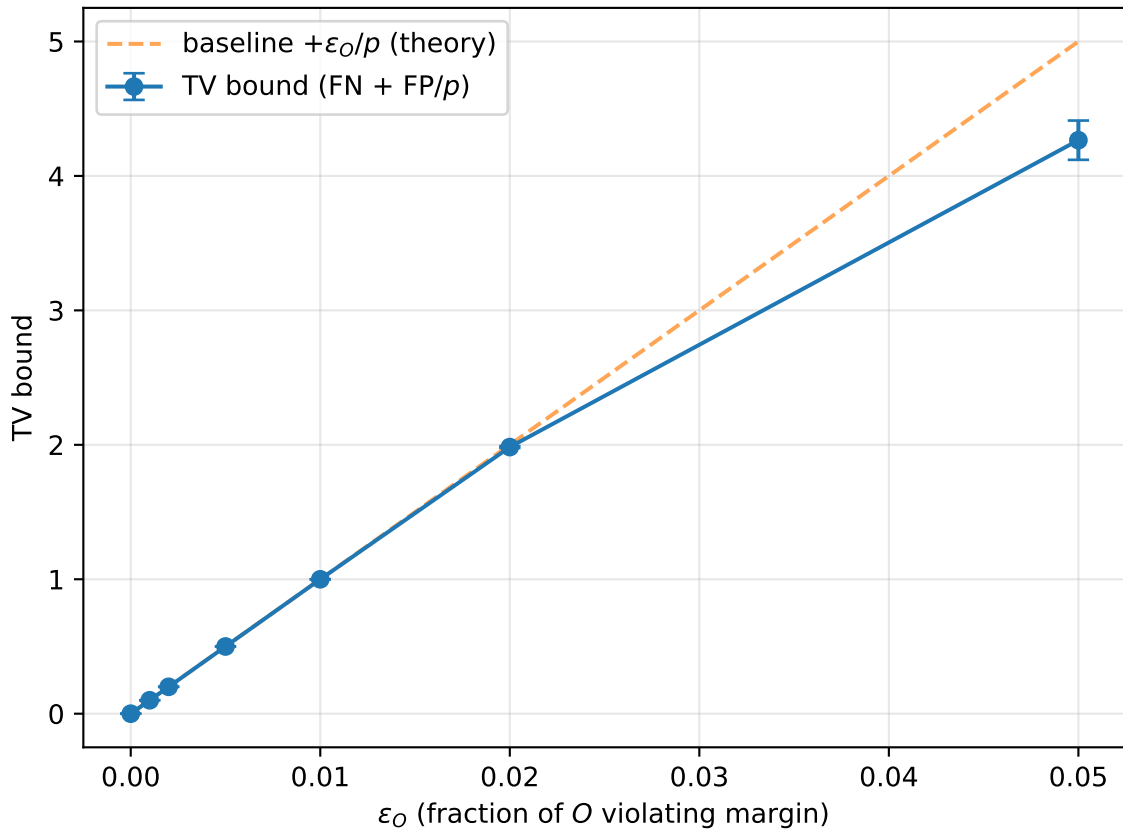
Weak separation: varying \varepsilon_O ( p = 0.01 )
