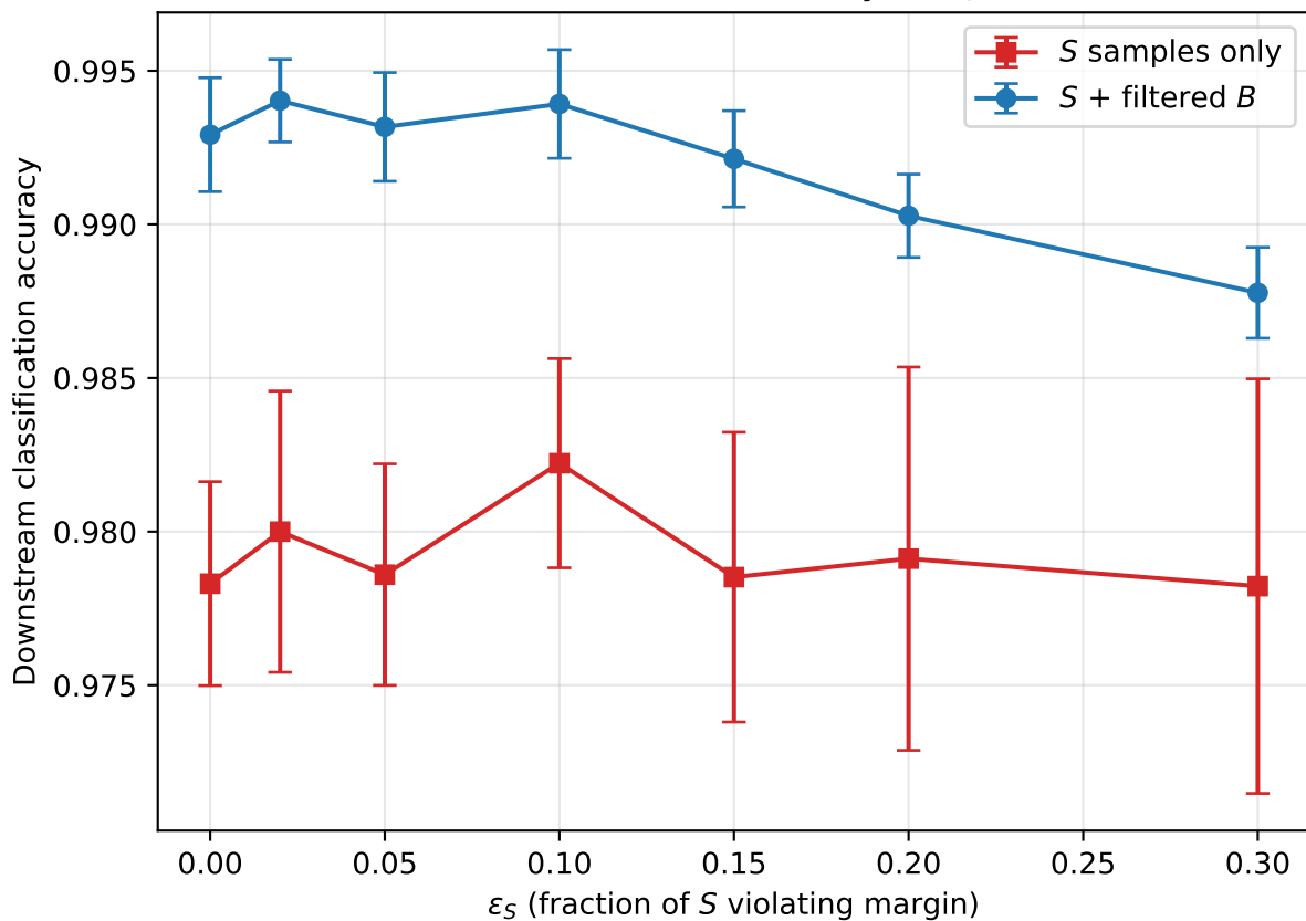
Downstream accuracy vs \varepsilon_S
