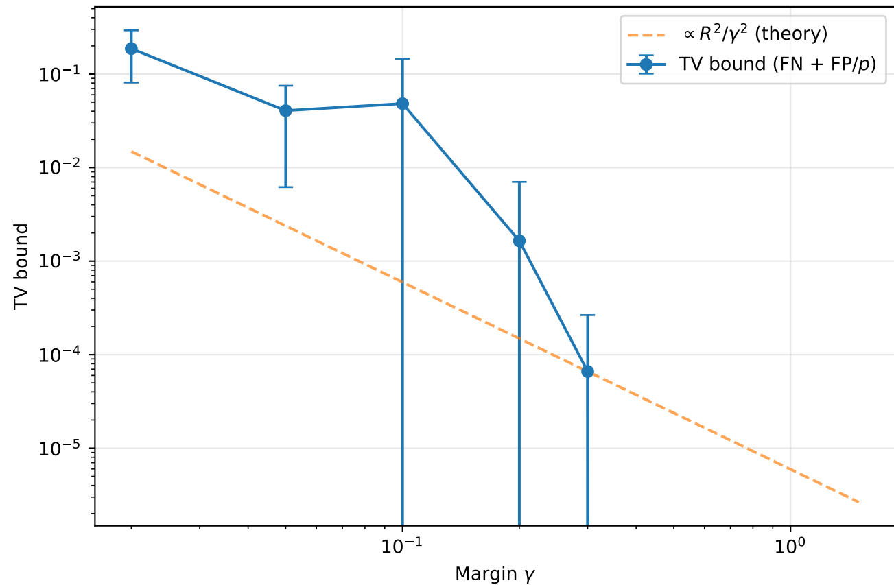
TV bound vs margin \gamma ( N_S = 30 , p = 0.01 , R = 3 )
