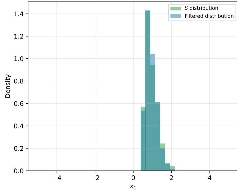
Distribution comparison (1st coordinate)
