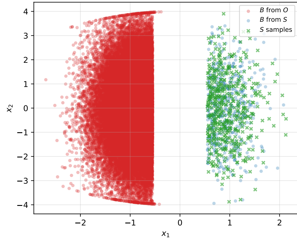
Input data (ground truth)
