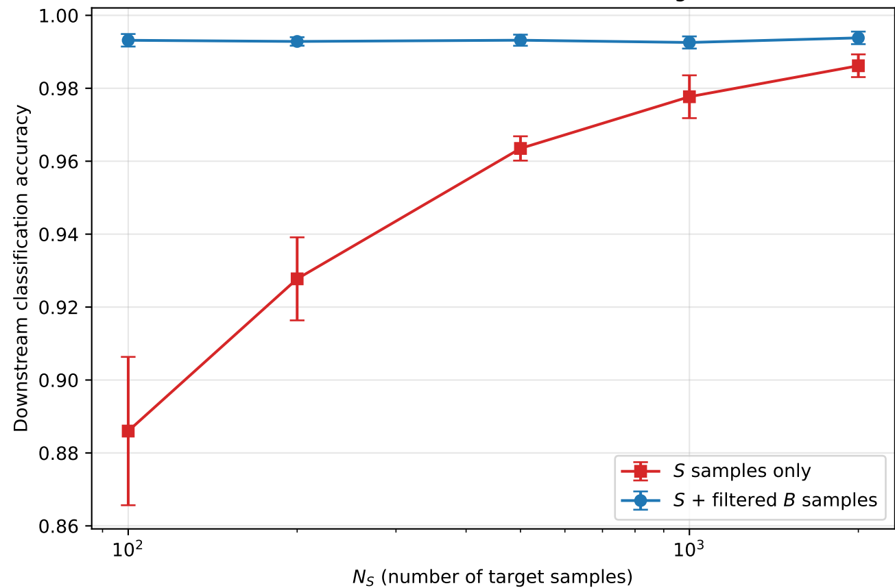
Downstream task: benefit of filtered data augmentation
