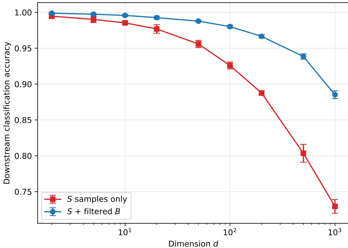
Downstream accuracy vs dimension d ( N_S = 1000 , p = 0.01 )
