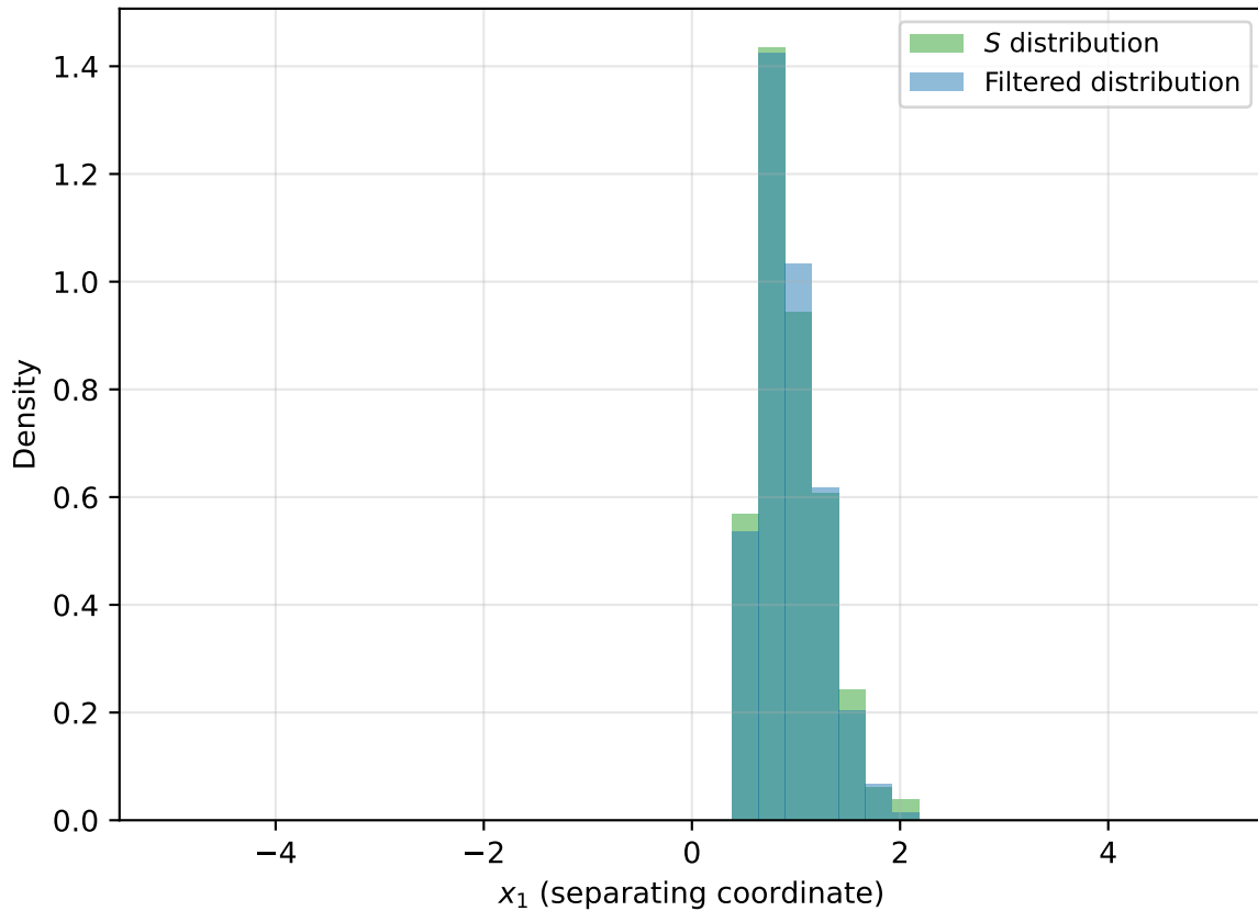
Distribution comparison (TV \approx 0.103 )
