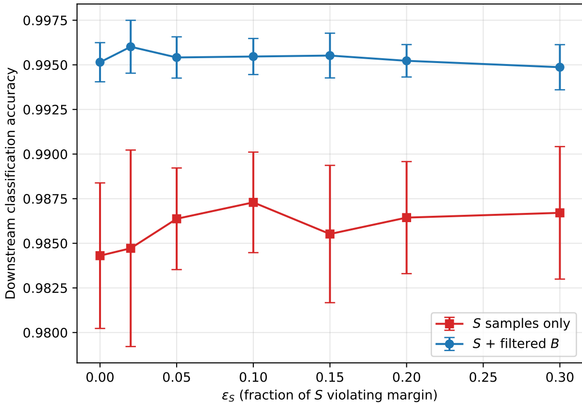
Downstream accuracy vs \varepsilon_S
